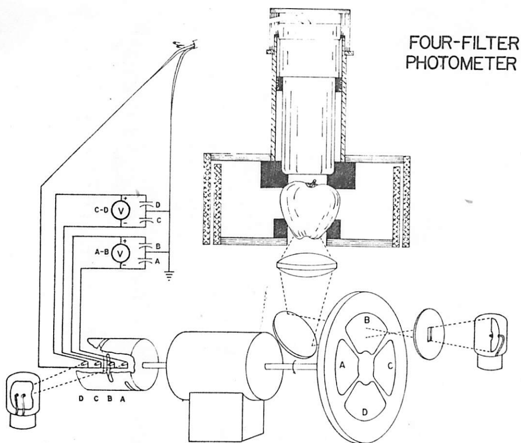
FIGURE 1.—Schematic of 4-filter difference meter.
