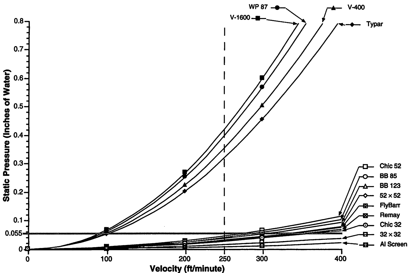
Figure 1. The resistance coefficient of a screening material as a function of static pressure and air velocity.
