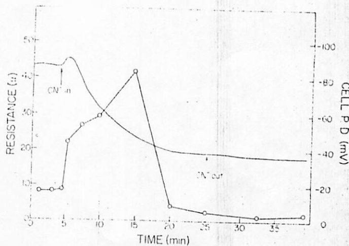
FIG. 4. Cyanide effect on pea root cortical cell. The electrical resistance ( \circ ) of a pea root cell as modified by \text{CN}^- during depolarization (—, cell PD). The drop in resistance at 15 min is believed to be a "punch-through" effect induced by the current pulses used for measuring R.
